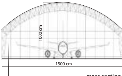
cross section
